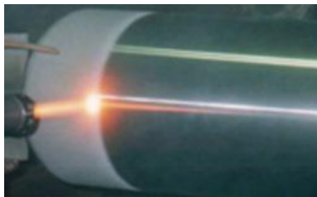
Cermet thermal spraying
